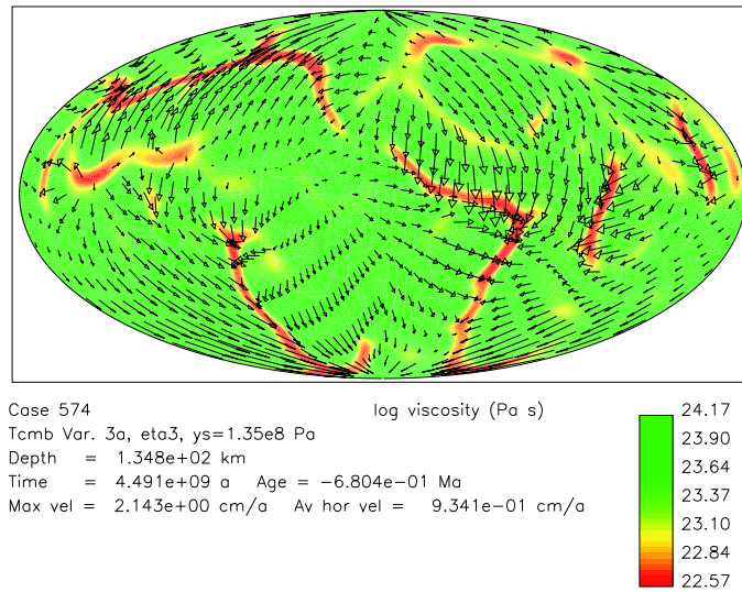
Figure 9. Equal-area projection of run 574 with \sigma_y = 135 MPa for the geological present. Arrows denote the creeping velocity, colors stand for the viscosity.
