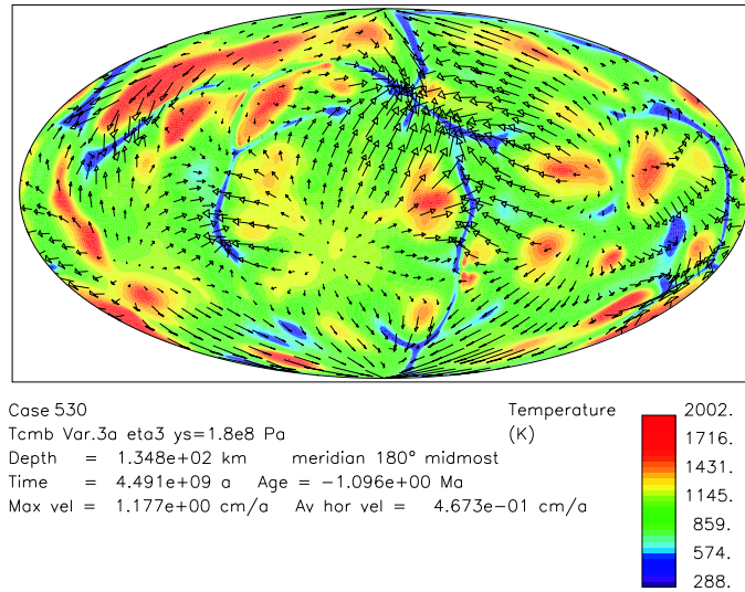
Figure 6. Equal-area plot of run 530 with \sigma_y = 180 \text{ MPa} in 134.8 km depth. This case is not plate like (See text).
